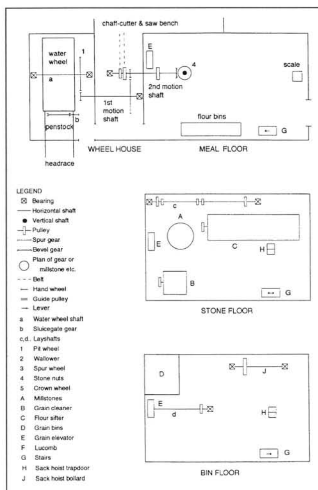
Fig. 5: Diagram of machinery layout in Connorville Mill.
