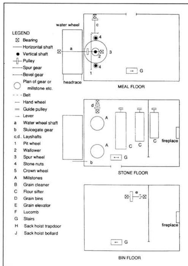
Fig. 10: Diagram of machinery layout, Millbrook Mill.
