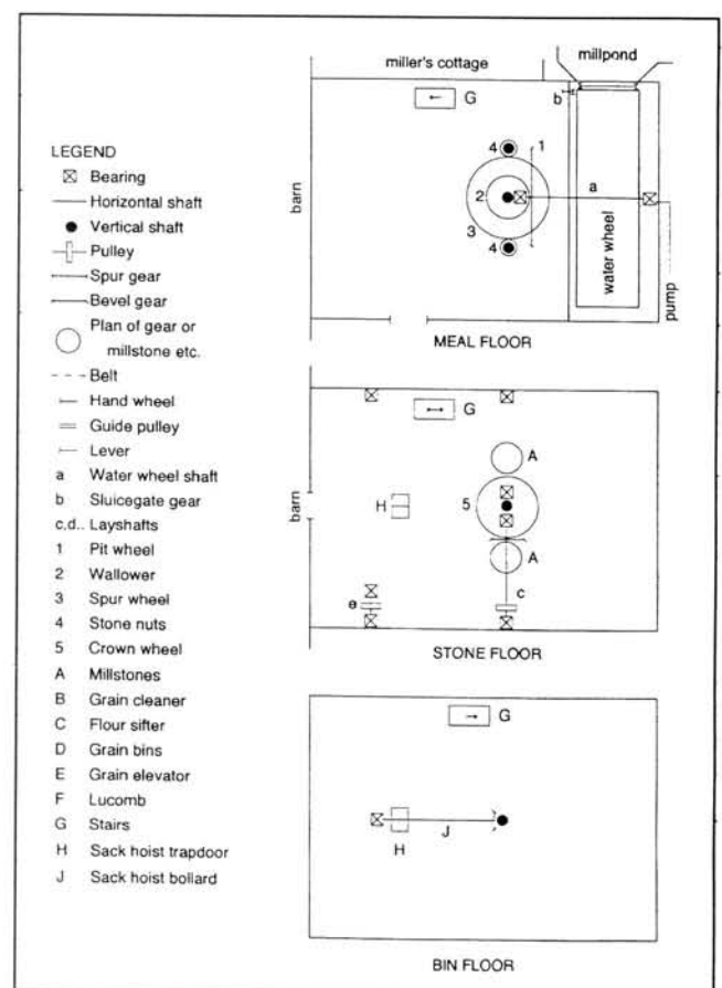
Fig. 8: Diagram of machinery layout, Nant Mill.
