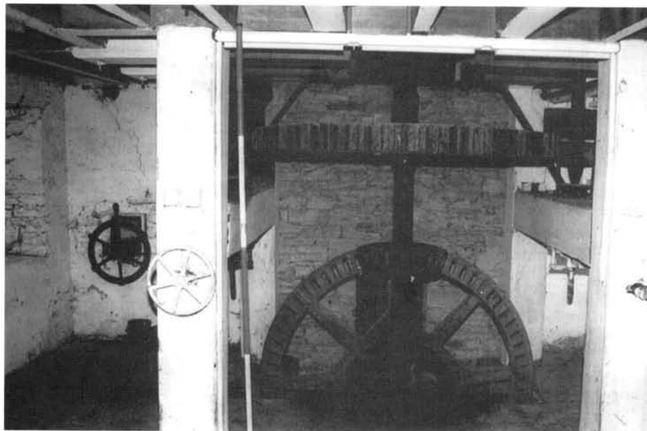
Fig. 7: Two-stage, underdrive gearing, Nant Mill. The screw jacks to engage the stone nuts, and bridgetrees for centering the millstones can also be seen. The hand wheel at left operates the sluiceway admitting water to the wheel (Photo W. Pearson, July 1993).
