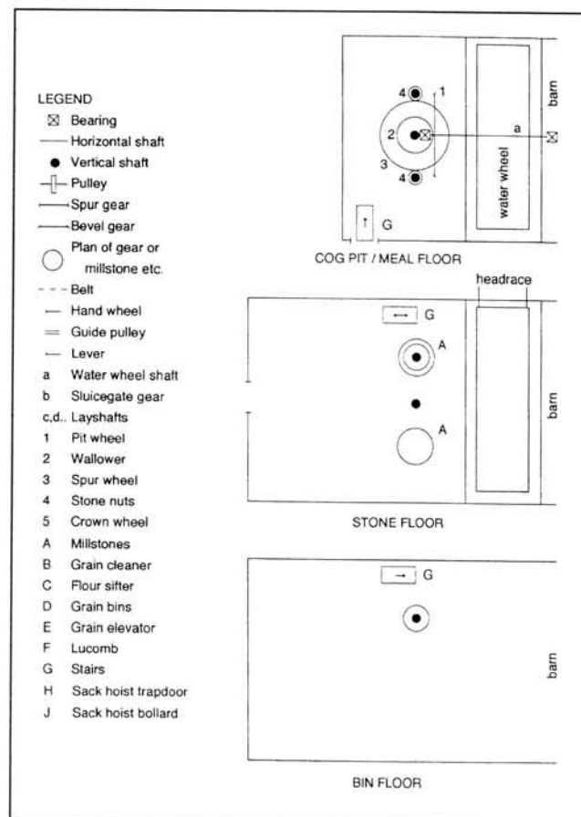
Fig. 9: Machinery layout diagram, Riversdale Mill.
