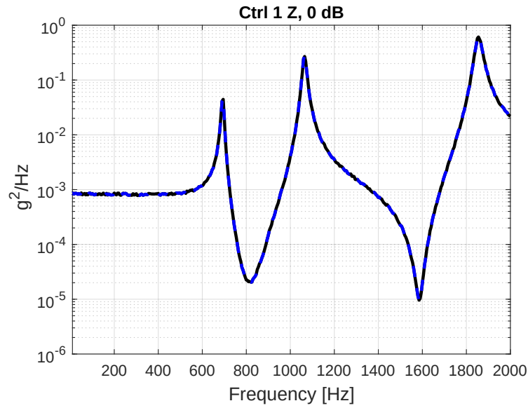
Figure 142: Control Accels, Noise, No CN, Case (4,1)
