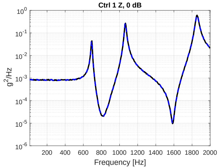
Figure 100: Control Accels, Noise, with CN, Case (3,1)
