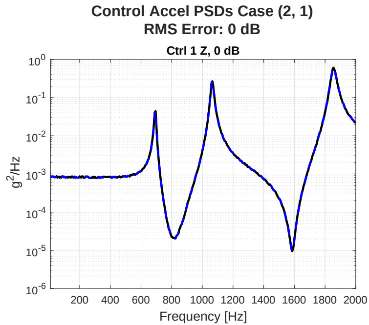
Figure 52: Control Accels, Noise, No CN, Case (2,1)
