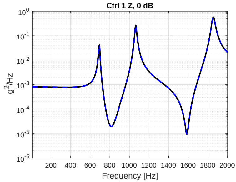
Figure 94: Control Accels, No Noise, Case (3,1)
