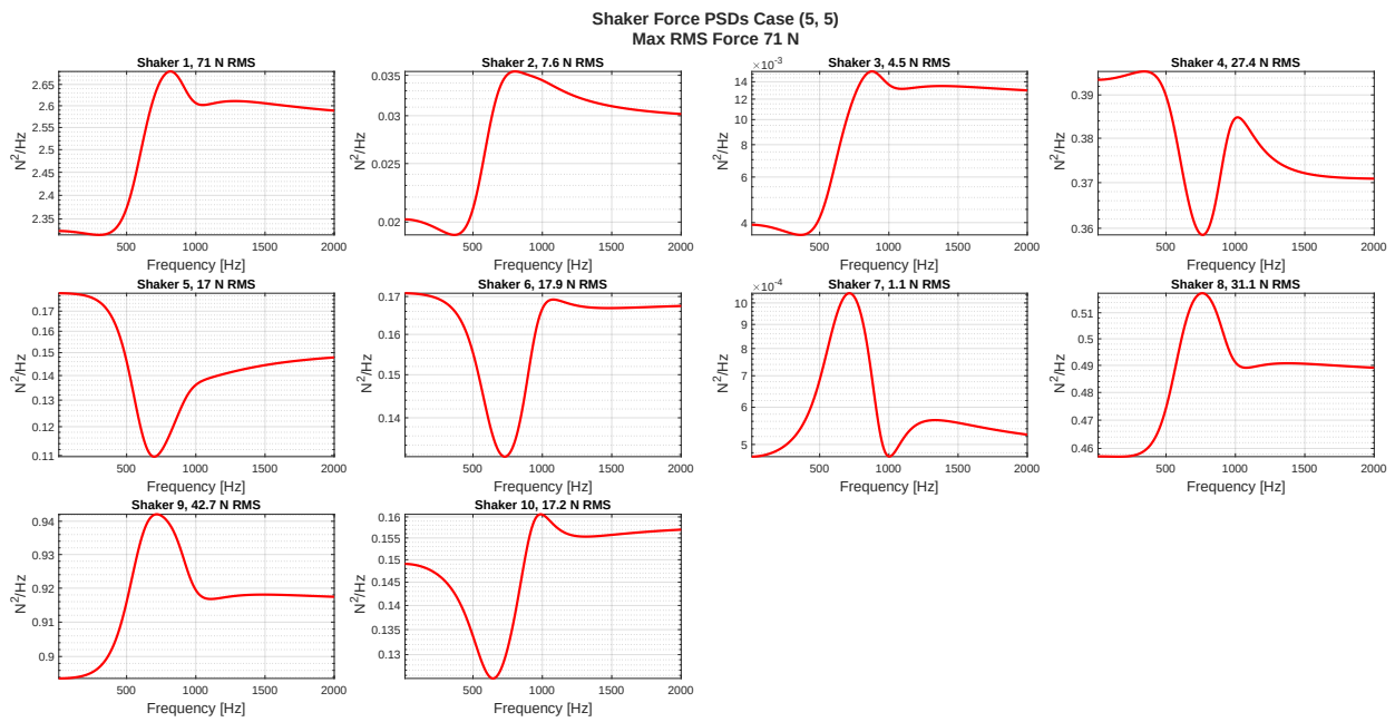
Figure 221: Shaker Forces, No Noise, Case (5,5)
